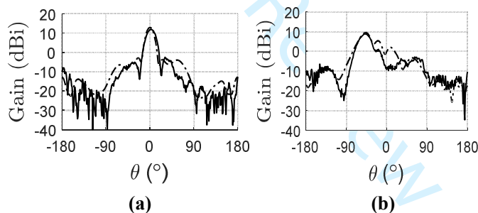
Figure 8. Radiation patterns, simulated (dash-dot line) and measured (solid line). (a) Boresight array (Taylor \beta = 0^\circ ). (b) Array steered to the maximum angle (Taylor \beta = 144^\circ ).
