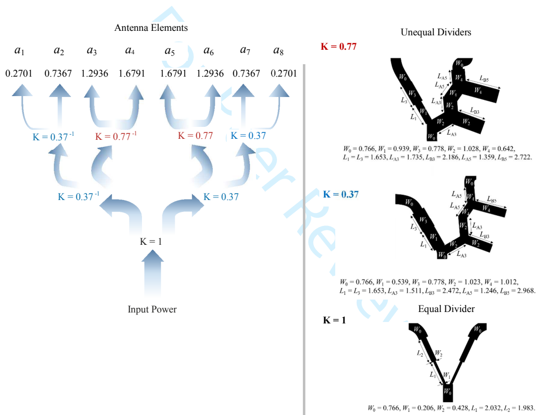
Figure 2. Voltage split ratios and unequal dividers within the feed network, to achieve the desired amplitudes. All physical dimensions are in mm.
