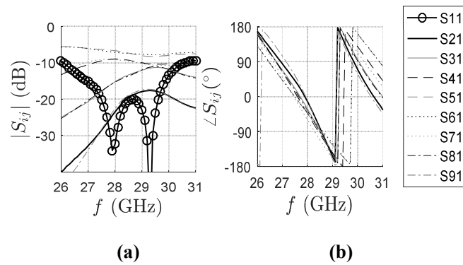
Figure 4. Taylor boresight feed network scattering parameter variation with frequency for all feed ports. (a) S parameter magnitudes. (b) S parameter phases, after correction.
