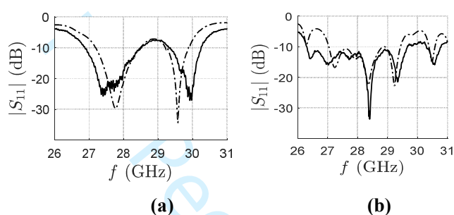
Figure 7. |S_{11}| , simulated (dash-dot line) and measured (solid line). (a) Boresight array (Taylor \beta = 0^\circ ). (b) Array steered to the maximum angle (Taylor \beta = 144^\circ ).
