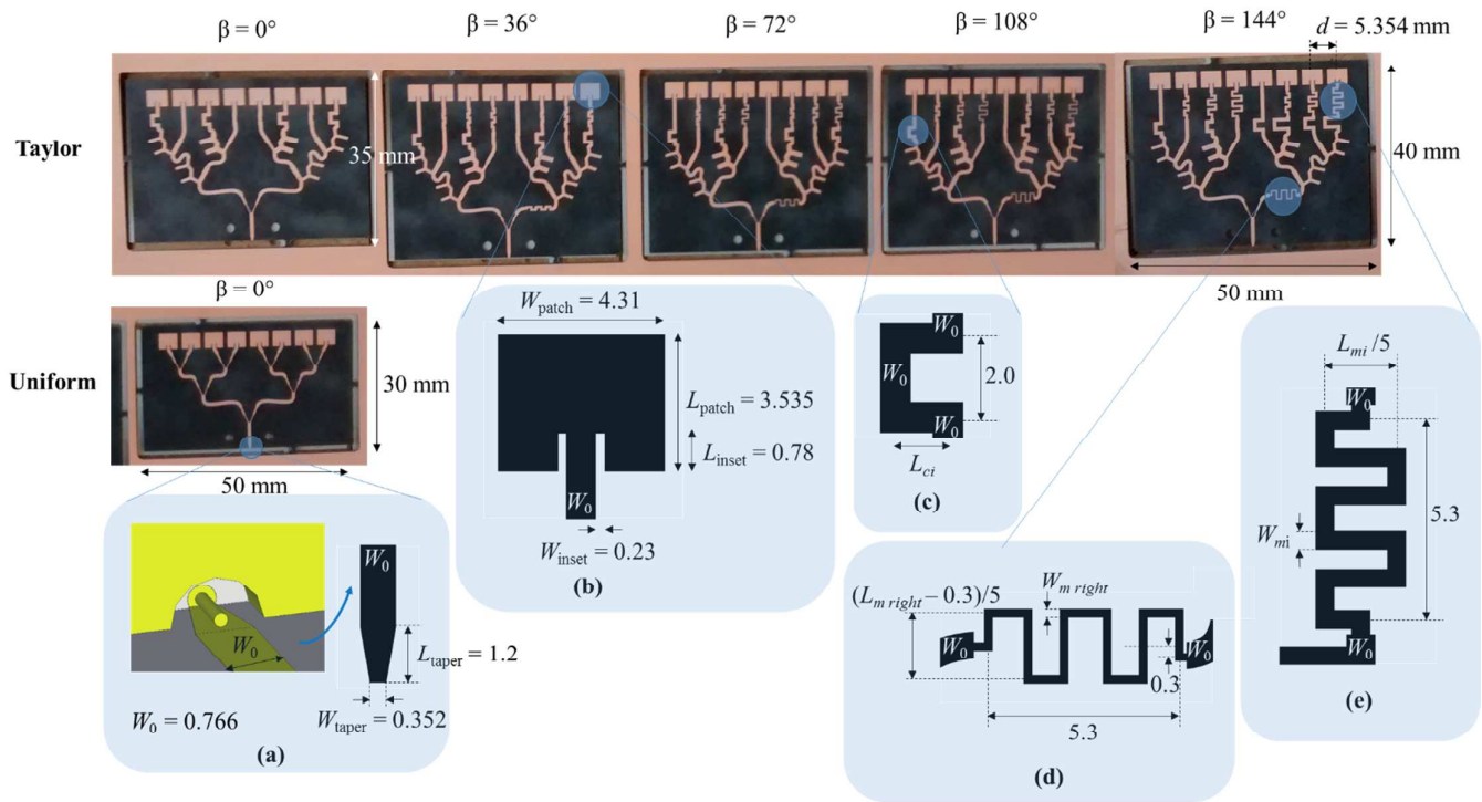
Figure 3. Photograph of the fabricated PCBs, with physical dimensions in mm. Inset: (a) Tapered transition. This introduces inductance to compensate for the capacitance of the 2.92 mm connector pin. (b) Patch element. Its dimensions were calculated as in Ref. [11], and W_{inset} was obtained by a parametric study. (c) Phase correction meander. (d) Right arm meander. (e) Beam steering meander.
