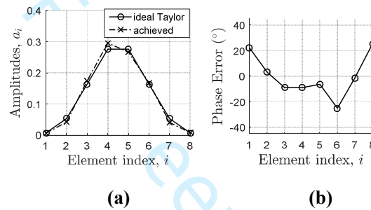
Figure 5. Achieved excitation at the feed output ports at 28 GHz. (a) Simulated and ideal Taylor amplitudes. (b) Phase error at the output of the feed, after correction.
