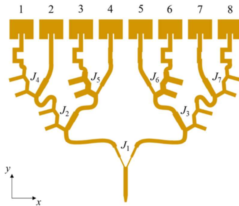
Figure 1. Proposed Taylor feed network (boresight). The transmission lines within the unequal dividers are much wider than for conventional unequal dividers.
