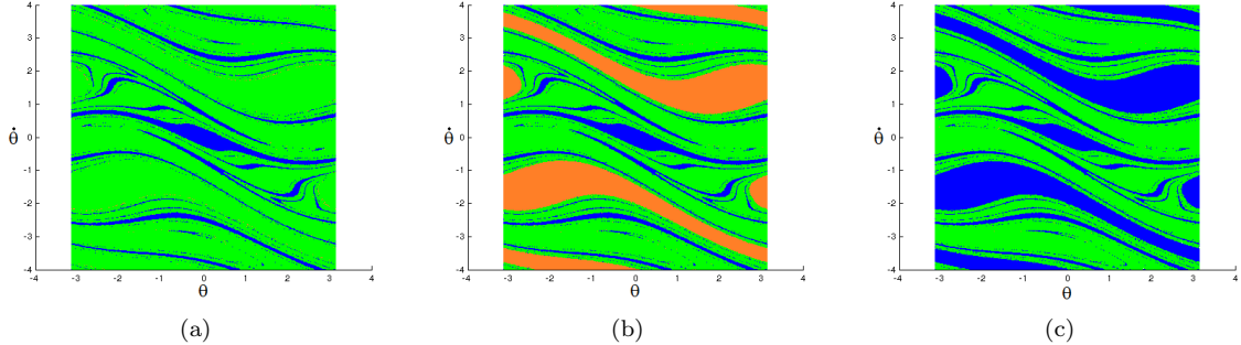
Figure 11: Basins of attraction for (1.2) with \alpha = -0.1 , \beta = 0.545 and \gamma(t) increasing linearly from \gamma_i = 0.23 to \gamma_f = 0.2725 over a time (a) T_0 = 93.6 , (b) 94.0 and (c) 99.2 . The colours are as in Figure 10.
