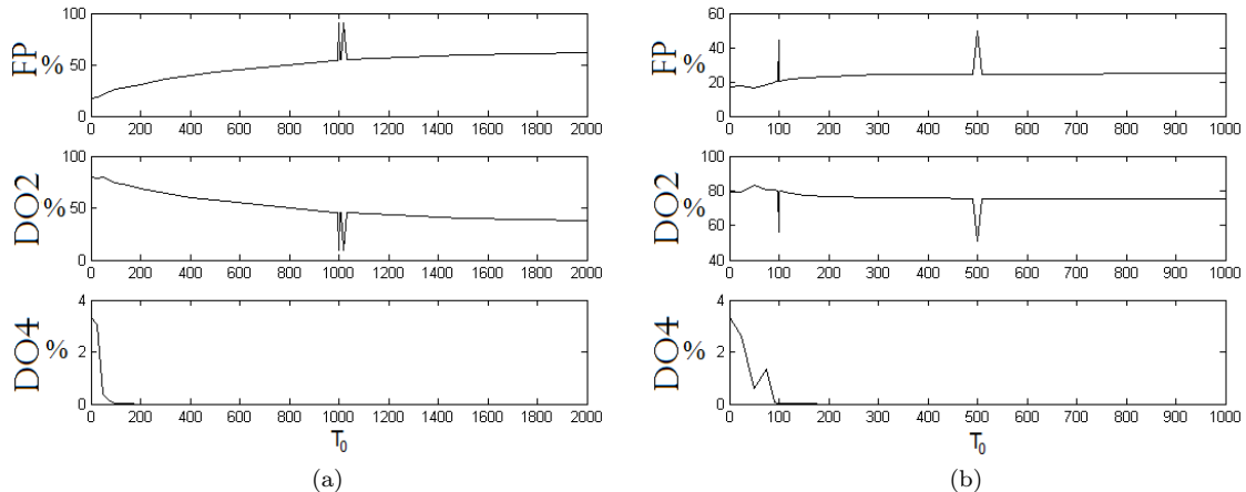
Figure 1: Relative areas of the basins of attraction for (1.2), with \alpha = -0.1 , \beta = 0.545 and \gamma(t) varying linearly over time T_0 from (a) \gamma_i = 0.2 and (b) \gamma_i = 0.23 to \gamma_f = 0.2725 . FP, DO2 and DO4 denote the persisting attractors: fixed point, period-2 oscillation and period-4 oscillation — see Section 4 for details.
