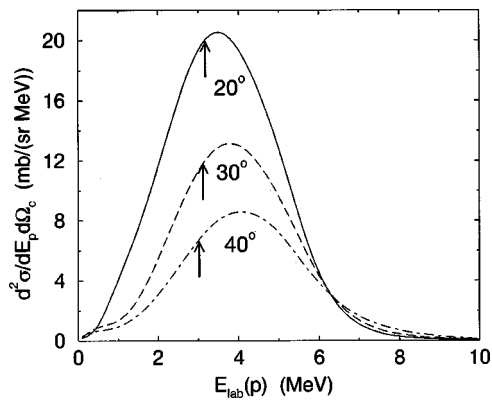
FIG. 10. Calculated laboratory-frame proton cross section energy distributions following the breakup of ^8\text{B} on ^{58}\text{Ni} at 25.8 MeV for the ^7\text{Be} fragment laboratory angles indicated. The calculations use the EB proton- ^7\text{Be} interaction and the BG proton-target interaction. The arrows indicate 1/8 of the ^8\text{B} energy for elastic scattering at each laboratory angle.
