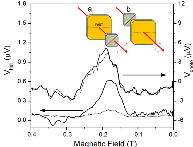
FIG. 10. (Color online) Confirmation that the signal detected at the modulation frequency is due to the degree of circular polarization. V_{photo} and V_{heli} are plotted for linear polarized incident light (solid lines) and circular polarized incident light (dotted lines). The only difference in the two optical arrangements is the position of the linear polarizer which is placed after the PEM to produce a linear polarized beam (a), and before the PEM to produce a circular polarized beam (b). Both V_{photo} and V_{heli} were recorded simultaneously at T = 10 K and \theta = 30^\circ .
