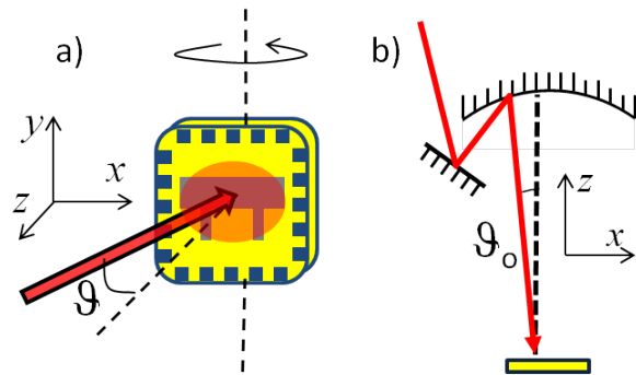
FIG. 2. Experimental setup. (a) Chip carrier can be rotated around y -axis, where the applied magnetic field direction is along the z -axis. \theta is the angle between the incident light and a vector normal to the device. (b) \theta = \theta_o when the plane of the QW is perpendicular to the z -axis.
