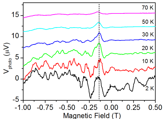
FIG. 4. (Color online) Temperature dependence of photoreponse using linearly polarized light. The plots have been offset by 3 \mu\text{V} for clarity. The dotted line indicates position of focusing signal in the dark at 135 mT. \theta = \theta_o .
