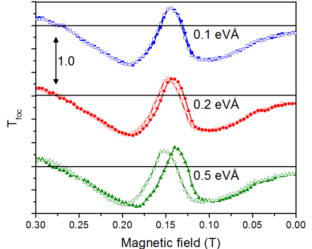
FIG. 8. (Color online) Calculated signal T_{foc} for focusing device shown in Fig. 7 for optical orientations of S_x = +1 (solid symbols) and S_x = -1 (open symbols), with \alpha = 0.1 \text{ eV\AA} (blue squares), 0.2 \text{ eV\AA} (red circles) and 0.5 \text{ eV\AA} (green triangles). N = 8000 for each data point.
