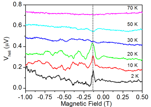
FIG. 5. (Color online) Temperature dependence of helicity signal using modulated circularly polarized light. The plots have been offset by 0.15 \mu\text{V} for clarity. The dotted line indicates position of focusing signal in the dark at 135 mT. \theta = \theta_o .
