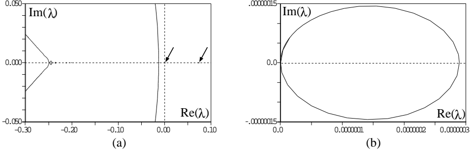
Fig. 6. (a) The essential spectrum of the slow periodic wave train at \epsilon = 0.0033 near the origin is plotted. The two tiny isolas located near \lambda = 0 and near \lambda = 0.08 have been enlarged to be visible. (b) Magnification of the isola which is attached to the origin.
