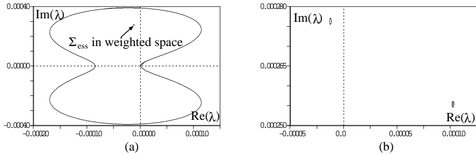
Fig. 5. (a) The isola from Figure 3(b) in the unweighted space and the upper part of the same isola, now computed in a weighted space with \text{Re} \nu \approx -0.035 . (b) Magnification of the isola in the weighted space for two different values of \epsilon : the unstable isola to the right corresponds to a value of \epsilon closer to the fold. Both isolas contain absolute spectrum, cf. [10].
