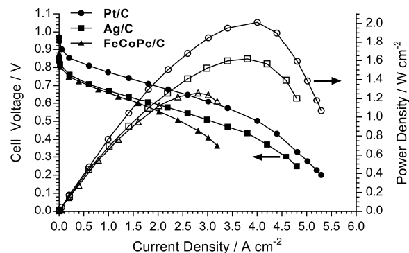
Fig. 6 H 2 /O 2 AEMFC performance data at 80 °C for LDPE15-AEM with the different cathode electrocatalysts. All other test conditions were as described in Fig 5 (including RH = 92% gas supplies).
