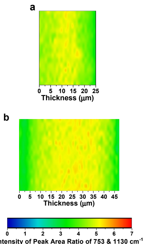
Fig. 2 Raman microscopic mapping through the core of a sample of (a) LDPE15-AEM and (b) LDPE15-AEM (both in the dehydrated \text{Cl}^- form). The through core direction is on the x-axis. The colour bars represent the ratios of the integrated area of the peak at 753 \text{ cm}^{-1} (relates to the ammonium groups) normalised to the area of the peak at 1130 \text{ cm}^{-1} (relates to the LDPE base material). Laser \lambda = 532 \text{ nm} (8 mW).
