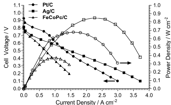
Fig. 8 H 2 /air(CO 2 -free) AEMFC performance data at 80 °C for LDPE15-AEM with the different cathode electrocatalysts. These H 2 /air(CO 2 -free) test were conducted immediately after the polarisation curves presented in Fig. 6 (without removal of the MEAs from the AEMFC). All other test conditions were as described in Fig 5 (including RH = 92% gas supplies).
