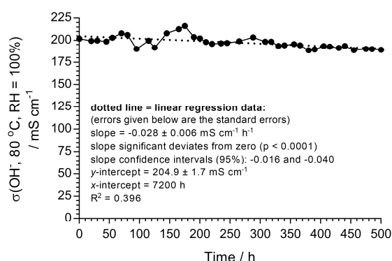
Fig. 3 A 500 h ex situ stability test with LDPE15-AEM in the OH - form at 80 °C in a N 2 (CO 2 -free, RH = 100%) gas flow. A d.c. current of 0.1 mA was used to maintain the OH - form of the AEM. Error! Bookmark not defined. The extended linear regression (to 3500h) is presented in Fig. S2 in the ESI + .
