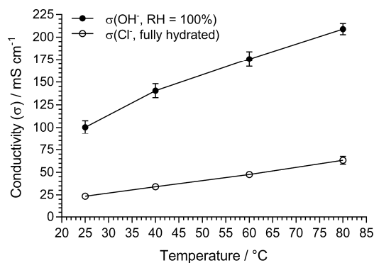
Fig. 1 The 4-probe (in-plane) conductivities of LDPE15-AEM under different conditions. Error bars are from measurements on n = 3 samples of each anion form of the AEM (some error bars are smaller than the symbols).
