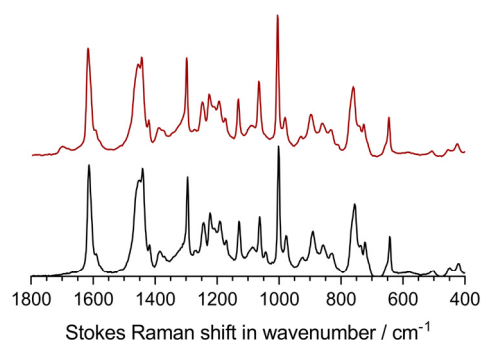
Fig. 4 The Raman spectra (λ = 532 nm) for LDPE15-AEM before (bottom – black) and after (top – red) the 500 h alkali stability test in Fig 3.
