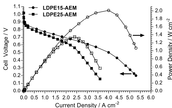
Fig. 5 H 2 /O 2 AEMFC performance data at 80 °C for LDPE15-AEM and LDPE25-AEM . PtRu/C (50% wt. Pt and 25% wt. Ru) anode and Pt/C (40% wt. Pt) cathode electrocatalysts were used and all electrodes contained Pt loadings of 0.4 \text{mg}_{\text{Pt}} \text{cm}^{-2} (geometric). All catalyst layers contained 20% wt. (solid mass) of a radiation-grafted ETFE powder ionomer (IEC = 1.26 \pm 0.06 \text{ mmol g}^{-1} ). All gases were supplied at 1 L \text{min}^{-1} with no back-pressurisation and RH = 92% (the gases used contained ca. 10 ppm CO 2 ).
