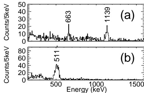
Figure 1. (a) Prompt GRETINA spectrum coincident with the identification of a ^{68}\text{Ni} recoil and the detection of a delayed 511-keV \gamma ray in the CsI(Na) focal plane detectors. (b) Delayed \gamma -ray spectrum recorded in the CsI(Na) scintillators in coincidence with implanted ^{68}\text{Ni} ions [18].
