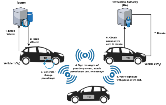
(b) DAA Pseudonym scheme lifecycle.
