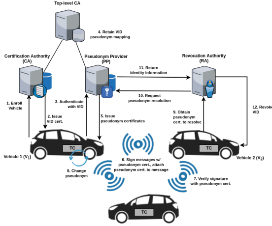
(a) Asymmetric Pseudonym scheme lifecycle. [10]
