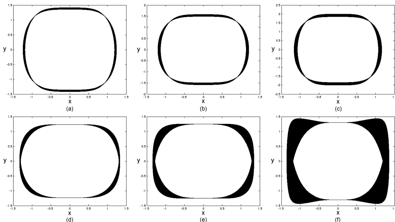
FIG. 3. Orbits for the system (1.2) with initial conditions (x, y) = (1, 1) . In (a)–(c) \omega = 0.0001 and in (d)–(f) \omega = 14 . The amplitude is \mu = 1 , in (a) and (d), \mu = 2 in (b) and (e), and \mu = 5 in (c) and (f).
