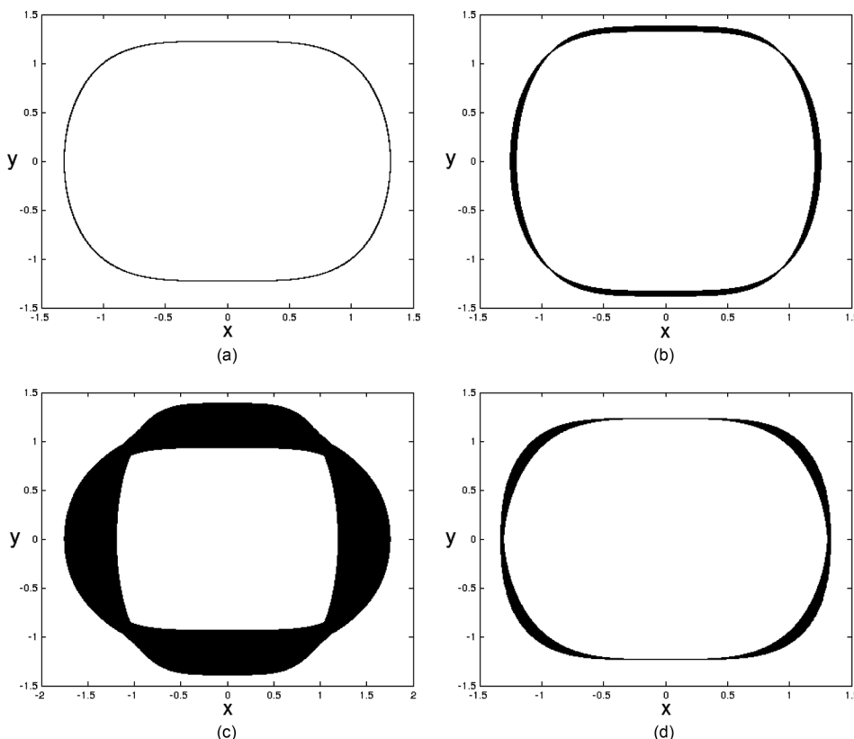
FIG. 1. Orbits for the system (1.2) with initial conditions (x, y) = (1, 1) . In (a) \mu = 0 . In (b)–(d) \mu = 0.8 and \omega = 0.0001, 0.2 , and 14 , respectively.
