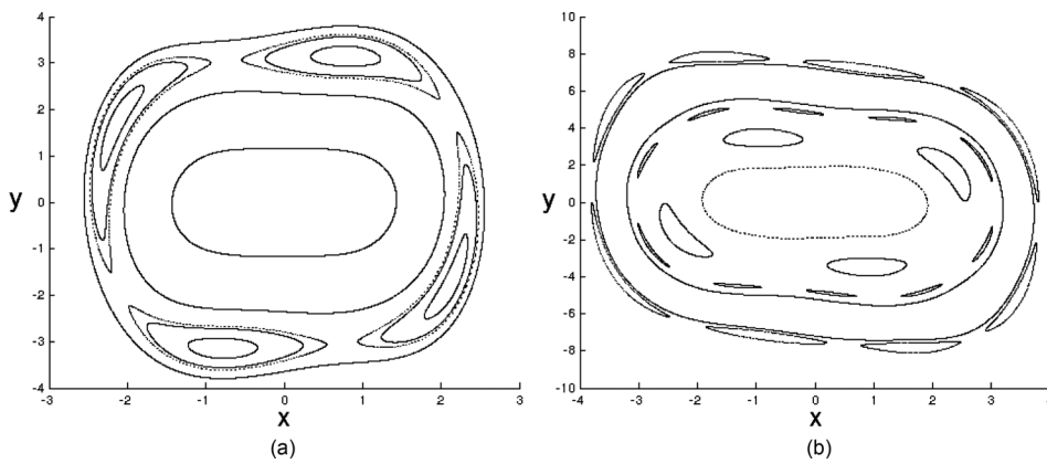
FIG. 2. Poincaré maps for the system (1.1) with \mu = 0.8 and various initial conditions, showing the break up of the KAM tori. The frequency is \omega = 0.2 and 0.4 in (a) and (b), respectively.
