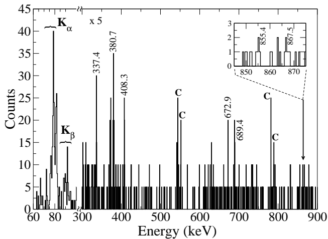
FIG. 6. The spectrum obtained from the sum of gates on the 408.3 and 689.4 \gamma -ray transitions in ^{209}\text{At} populated via \alpha -decay of ^{213}\text{Fr} . The inset illustrates the evidence of the 855.4 and 867.5 keV \gamma rays and the letter “C” denotes contaminant \gamma rays known from the decay of ^{209}\text{At} .
