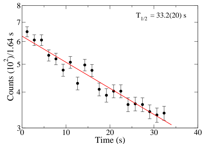
FIG. 4. (Color online) Fit to the decay of the 605.9 keV conversion electrons corresponding to 704.3 keV \gamma rays in ^{213}\text{Rn} which is populated in the \text{EC}/\beta^+ decay of ^{213}\text{Fr} .
