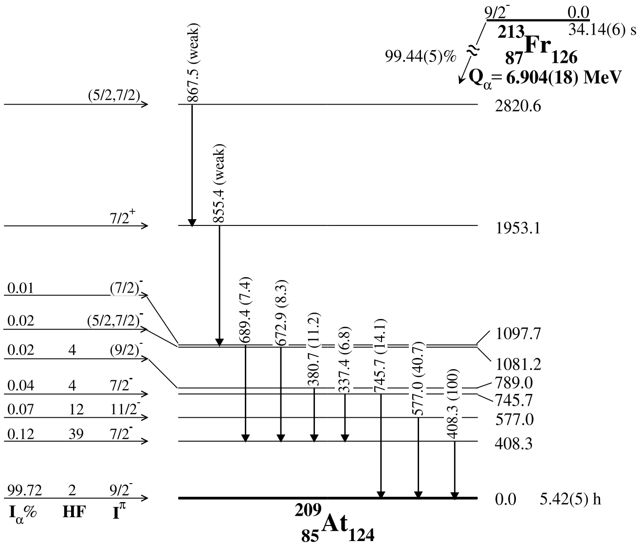
FIG. 8. Level scheme of ^{209}\text{At} as obtained from the \alpha -decay of ^{213}\text{Fr} . All the transitions are labeled with their energies. The numbers on the left side indicate the spin-parity, relative \alpha -decay intensity, and hindrance factor; while those on the right side indicate the excitation energy of each level in keV. The spin-parity values and the ground-state half-life of ^{209}\text{At} are taken from Ref. [38]. The ground-state half-life and \alpha -decay Q value of ^{213}\text{Fr} are from Refs. [28] and [34], respectively.
