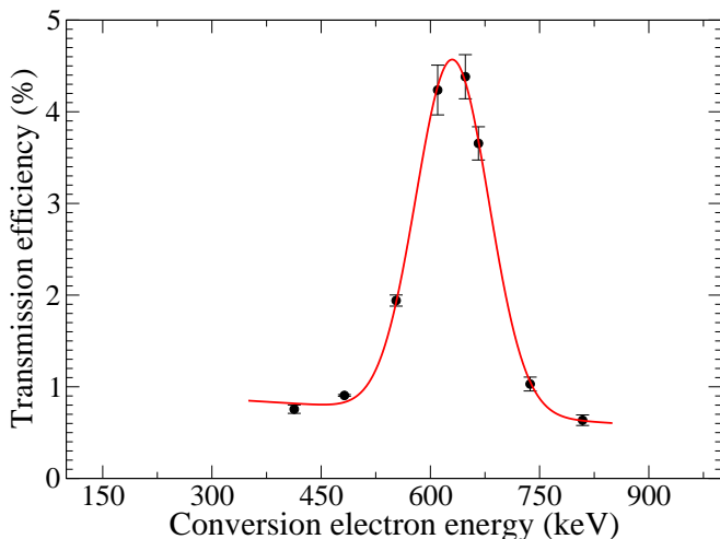
FIG. 1. (Color online) Transmission efficiency curve of the MINI-ORANGE spectrometer.
