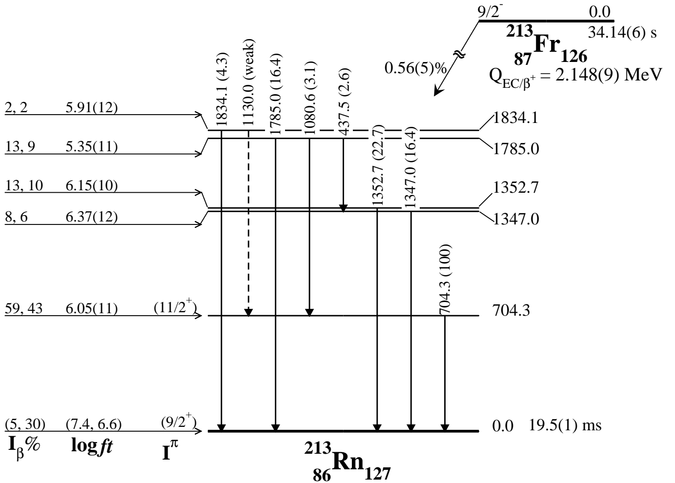
FIG. 5. Level scheme of ^{213}\text{Rn} as obtained from the \beta -decay of ^{213}\text{Fr} . All the transitions are labeled with their energies and relative \gamma -ray intensities in brackets. The numbers on the right indicate the excitation energy of each level in keV. The EC/ \beta^+ branching ratio of ^{213}\text{Fr} and ground-state half-life of ^{213}\text{Rn} are from Ref. [13]. The ground-state half-life and the EC/ \beta^+ -decay Q value of ^{213}\text{Fr} are from Refs. [28] and [34], respectively.
