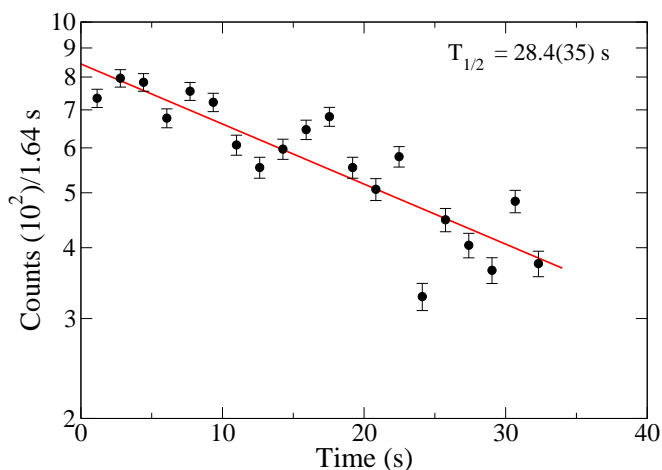
FIG. 7. Fit to the decay of the 577.0 keV \gamma ray in ^{209}\text{At} populated via \alpha -decay of ^{213}\text{Fr} .
