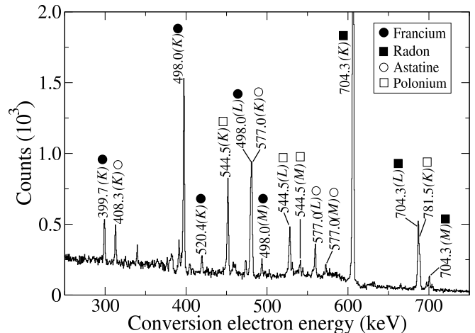
FIG. 2. Part of the singles conversion electron spectrum, illustrating transitions from excited states in ^{213}\text{Fr} , ^{213}\text{Rn} , ^{209}\text{At} , and ^{209}\text{Po} with the A = 213 GPS setting. The transitions are labeled with the corresponding \gamma -ray energies.
