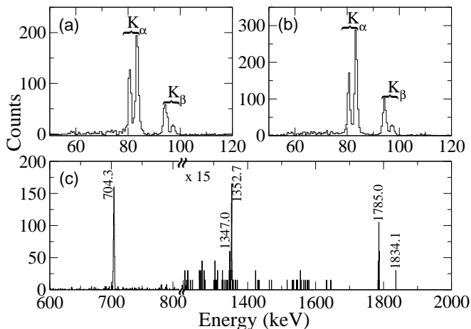
FIG. 3. Spectra showing radon K_\alpha and K_\beta x rays obtained with gates on (a) 704.3 keV events from the \gamma-\gamma matrix and (b) 605.9 keV conversion electrons (corresponding to 704.3 keV \gamma rays) from a \gamma -ray-conversion-electron matrix. Fig. (c) shows \gamma -ray spectra obtained from adding K_{\alpha_1} , K_{\alpha_2} , and K_{\beta_1} radon x-ray gates using the \gamma-\gamma matrix.
