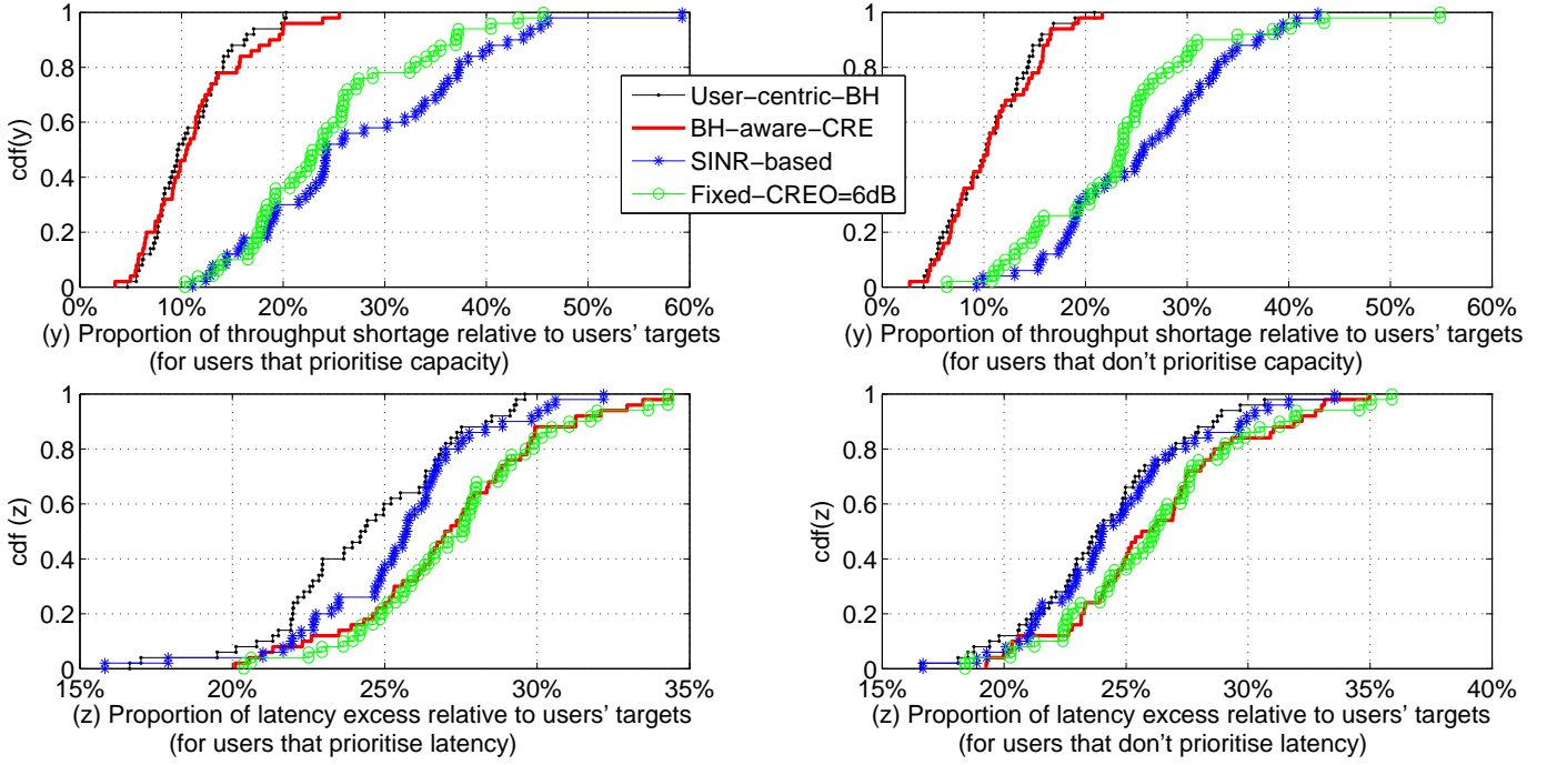
Fig. 3. The upper figures show the shortage in achievable system throughput relative to the cumulative users' targets, looking at users that associate a high weight to throughput (upper-left) and those that do not (upper-right). The lower figures show the excess in achievable latency relative to the users' targets, looking at users that associate a high weight to latency performance (lower-left) and those that do not (lower-right).
