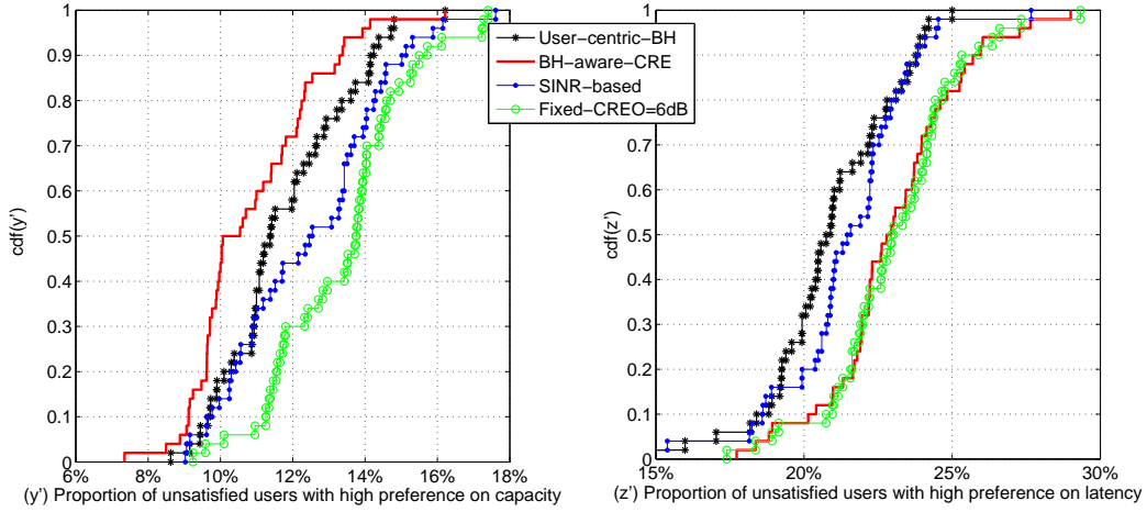
Fig. 2. Percentage of unsatisfied users with respect to throughput, y' , (Left) and latency, z' , (Right). The novel User-centric-BH scheme compares to the BH-aware-CRE with respect to throughput QoS but results in major improvements with respect to latency related QoS.
