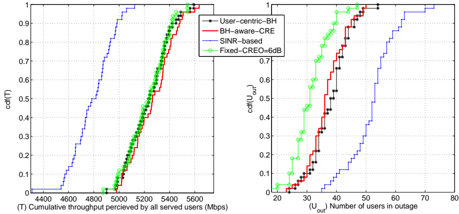
Fig. 1. (Left) Cumulative users' throughput and (Right) Number of users in outage. CRE-based schemes outperform SINR-based and the novel User-centric-BH compares closely to the BH-aware-CRE in these performance indicators.
