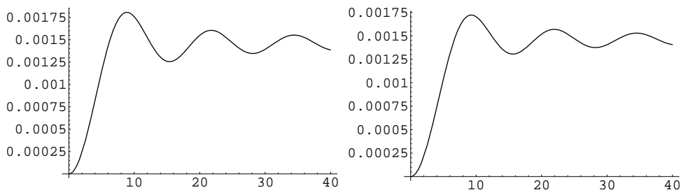
Figure 6: The imaginary parts \Im\widehat{\Pi}_c(q) and \Im\{\widehat{\Pi}_c + \widehat{\Pi}_\vartheta\} as functions of |\tilde{q}| , for g^2 = 10^{-2} .
