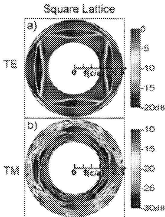
Transmission as a function of f/f_c and angle \theta
