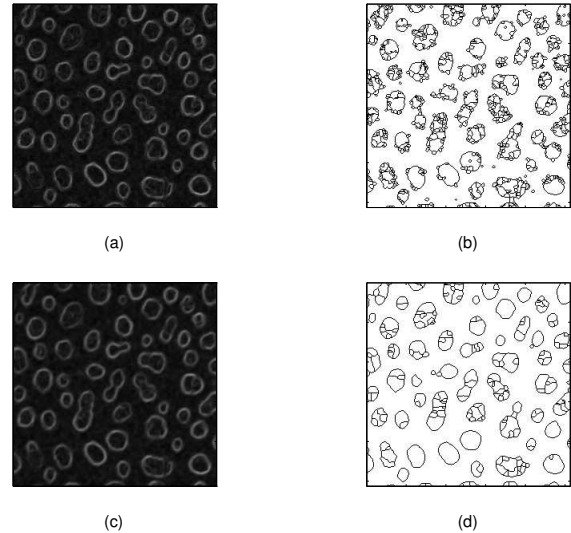
Figure 6: a)One-stage gradient of noisy Cermet ; b)Detected contours of a); c)Two-stage gradient of noisy Cermet ; d)Detected contours of c).
