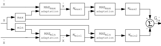
Figure 3: Two-stage of Difference of Estimates
