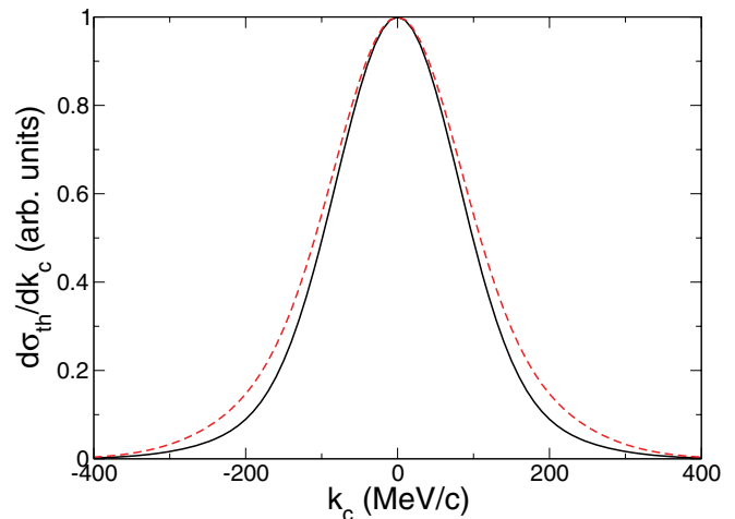
FIG. 2. (Color online) Calculated inclusive longitudinal momentum distributions in the projectile rest frame for (i) reactions to all final states (solid curve) and (ii) for all events with a coincident 2_1^+ -state \gamma ray (dashed curve). Calculations use the SDPF-MU shell-model TNAs. These momentum distributions are normalized to unity at their peaks.
