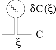
Figure 1: A single propagator inserted in the small loop
