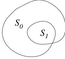
Figure 3: A loop with two windows
