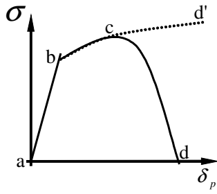
Figure 1 - A damaged material response based on the equivalent plastic displacement using the continuum damage failure model
