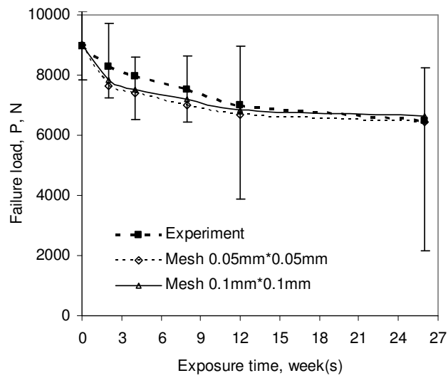
Figure 10 - Predicted ultimate failure load of the EA9321/aluminum SLJ using the continuum damage model
