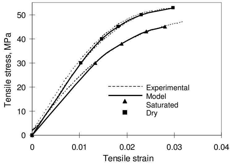
Figure 2 - Moisture dependent tensile properties of bulk EA9321
