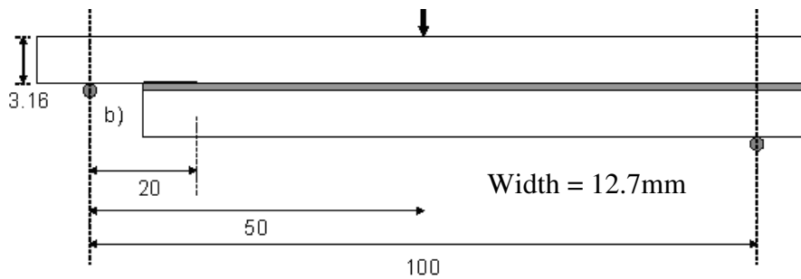
Figure 3 - Geometry and loading configuration of the MMF specimen
