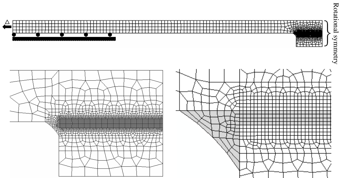
Figure 9 - FE model of the EA9321/aluminum SLJ and local mesh refinement
