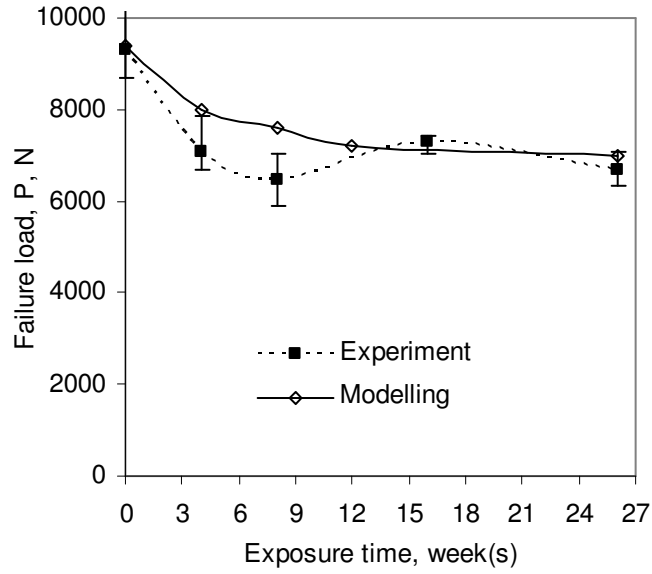
Figure 13 - Predicted ultimate failure load of the EA9321/composite SLJ using the continuum damage model (smallest mesh size 0.05mmx0.05mm)
