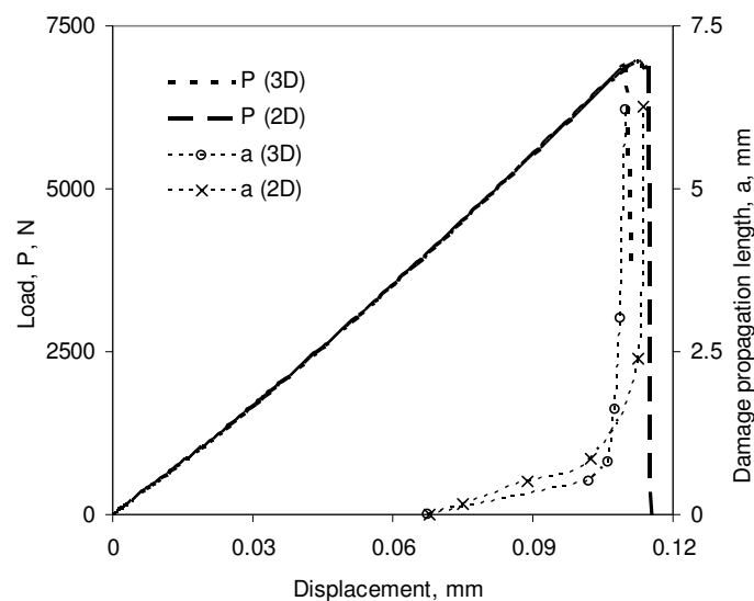
Figure 20 - Predicted loading history and damage propagation in a 3D and 2D EA9321/composite SLJ model after exposure for 26 weeks
