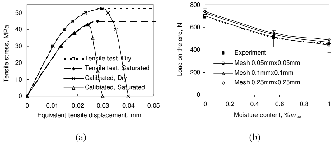
Figure 8 - The mesh independent, moisture dependent damage curves calibration: (a) Calibrated results; (b) Predicted failure loads of the MMF specimen
