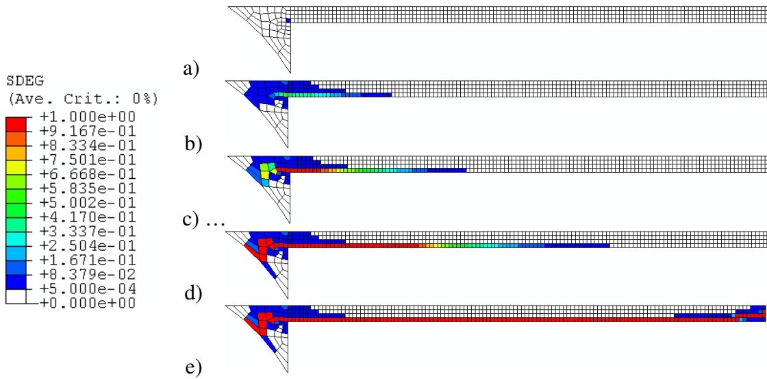
Figure 11 - Damage propagation in the EA9321/aluminum SLJ model (26weeks degraded)
