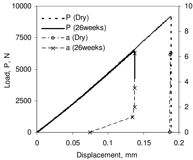
Figure 12 - Predicted loading history and damage propagation in an undegraded joint and a joint aged for 26 weeks (EA9321/aluminum SLJ, smallest mesh size 0.05mmx0.05mm)
