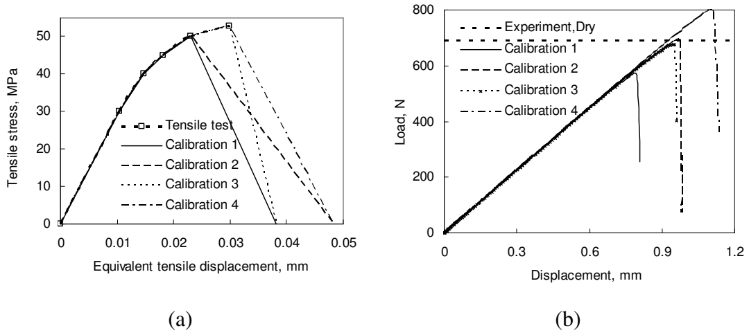
Figure 7 - The damage curve calibrations of dry EA9321 using the MMF model (smallest mesh size 0.1mmx0.1mm): (a) Calibration curves (of unit-size elements); (b) Predicted loading history
