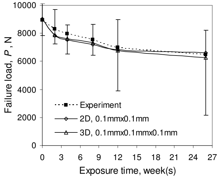
Figure 17 - Predicted ultimate failure load of the EA9321/aluminum SLJ using the continuum damage 2D and 3D model
