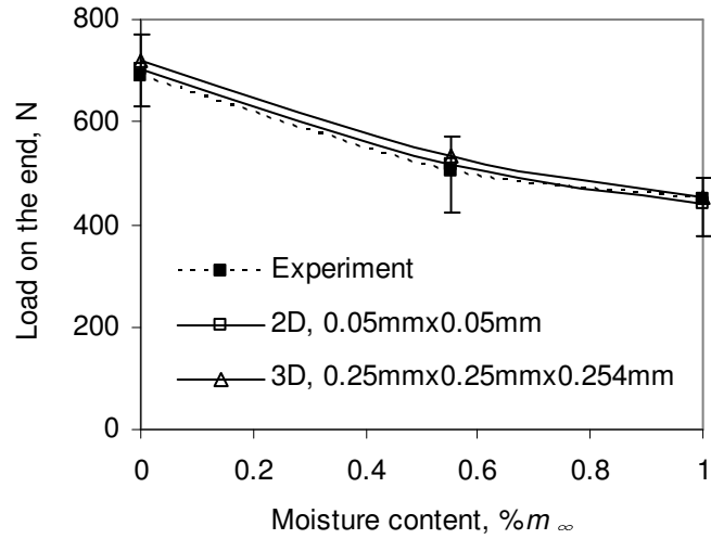
Figure 15 - Predicted failure loads from the 2D and 3D MMF models using the continuum damage model with the different mesh sizes
