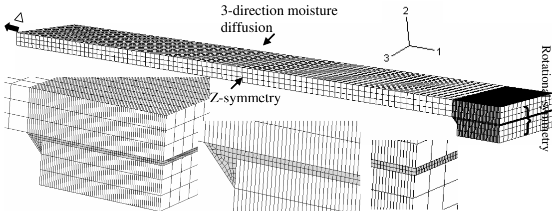
Figure 16 - 3D quarter symmetrical model of the EA9321/aluminum SLJ and local mesh refinement (smallest mesh size: 0.1mmx0.1mmx0.1mm)
