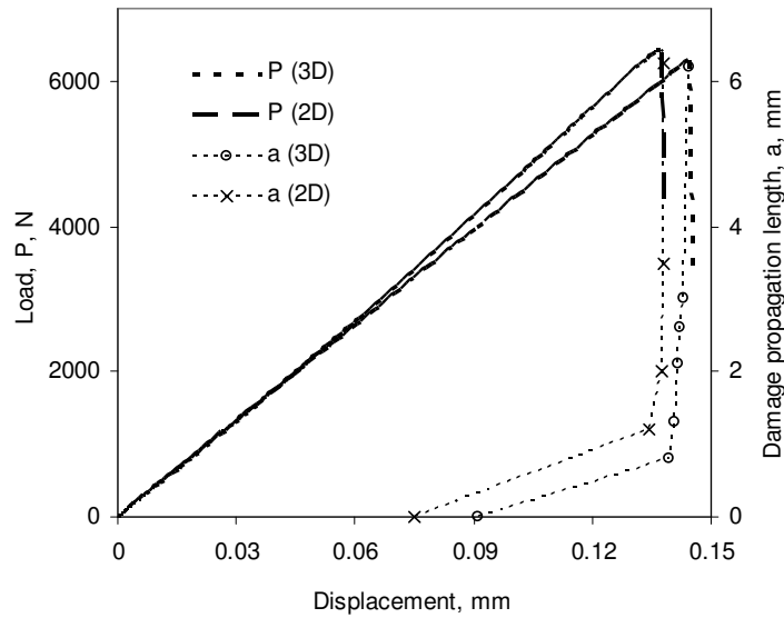
Figure 18 - Predicted loading history and damage propagation in a 3D and 2D EA9321/aluminum SLJ model after exposure for 26 weeks
