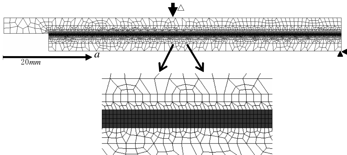
Figure 6 - MMF FE model with mesh refinement along the adhesive overlap
