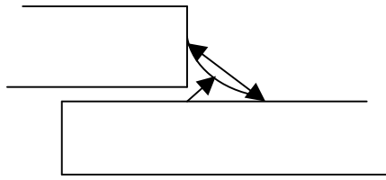
Figure 4 - Fillet configuration of the EA9321 bonded SLJs (not to scale)
