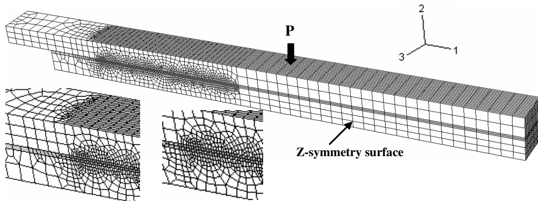
Figure 14 - 3D model of the MMF test and local mesh refinement used for the continuum damage model (smallest mesh size: 0.25mmx0.25mmx0.25mm)
