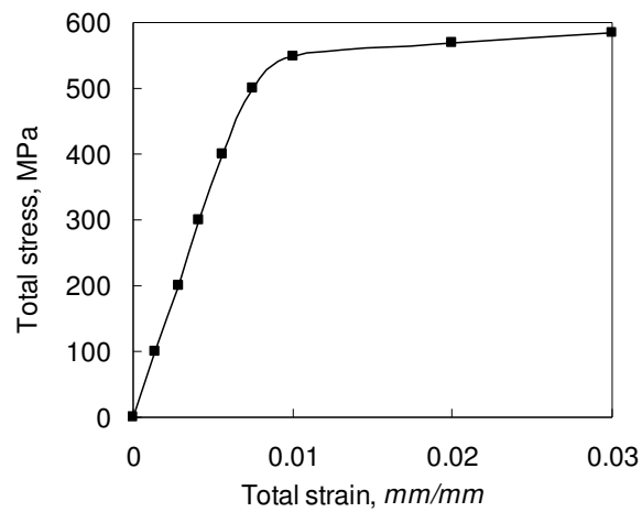
Figure 5 - Tensile properties of aluminum substrates ( E = 72\text{GPa} , \nu = 0.3 ) [26]
