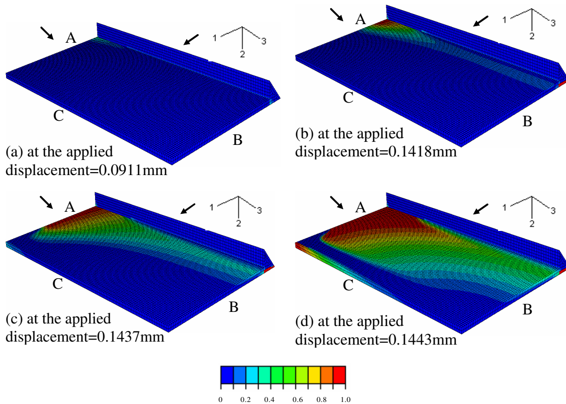
Figure 19 - 3D damage propagation in the EA9321/aluminum SLJ model using the continuum damage model (26 weeks degraded)
