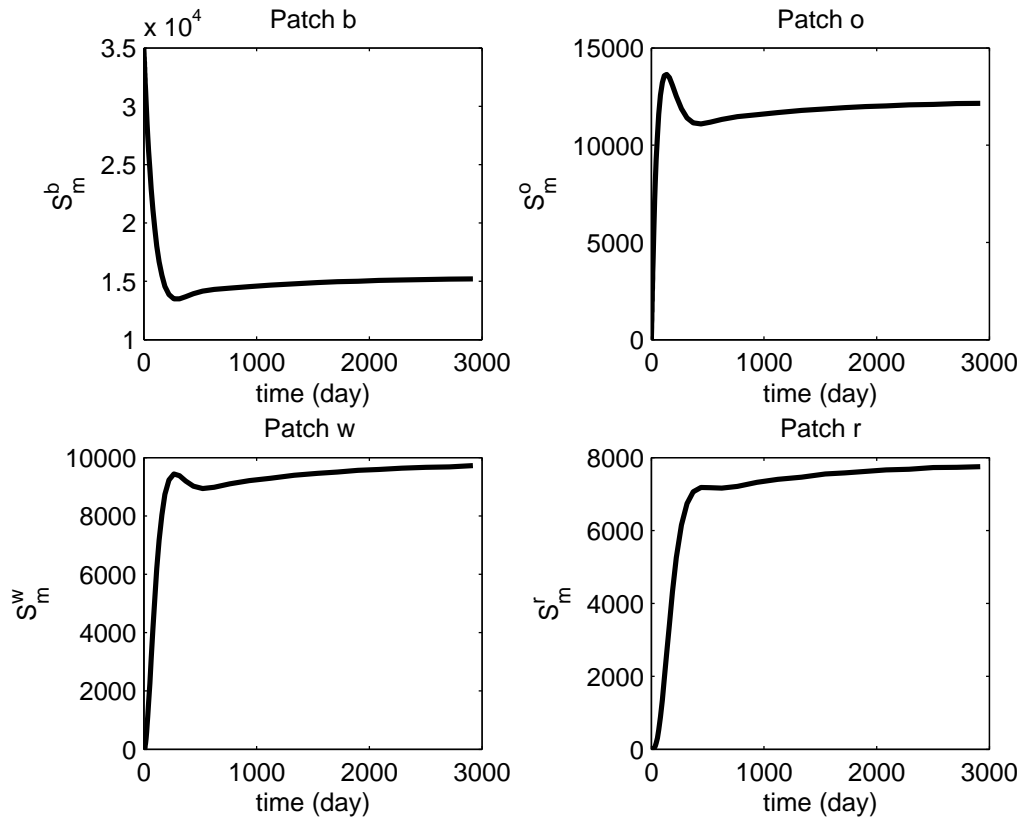
Figure 1: The solution of system (4.23) goes to the positive equilibrium if assumption (H1) holds.
