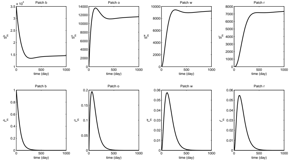
Figure 2: Stability with poultry absent. This figure demonstrates that if assumption (H1) and inequality (4.27) are satisfied, the disease free nontrivial equilibrium of the system with poultry absent is stable. Here \beta_m^j = 5 \times 10^{-7} for each j = b, o, w, r .
