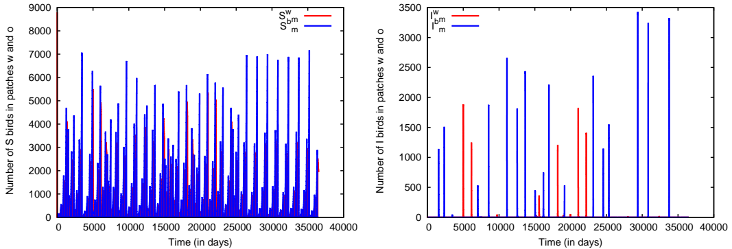
Figure 7: Number of (left) susceptible and (right) infected migratory birds over 100 years in the absence of poultry showing disease persistence and appearance of non-periodic oscillation of the number of migratory birds. Here, I_m^w(0) = 10 , S_m^w(0) = 8800 , \beta_m = 1.5 \times 10^{-4} \text{day}^{-1} , r = 15,000 , \gamma = 0.0146 \text{day}^{-1} , \mu_{ms} = 0.0022 \text{day}^{-1} , and \mu_{mi} = 0.23 \text{day}^{-1} . The death rates in flight are taken to be equal to those on land.
