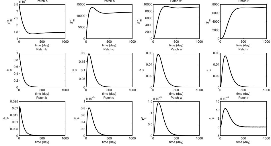
Figure 4: This figure shows that if assumptions (H1, H2) and inequalities (4.25), (4.27) and (4.28) hold, then the disease free nontrivial equilibrium of system (2.4)-(2.5) is globally asymptotically stable. Here, \beta_m^j = 5 \times 10^{-7} , \beta_j^p = 8 \times 10^{-7} , \beta_{mp}^j = \beta_{pm}^j = 5 \times 10^{-9} for j = b, o, w, r .
