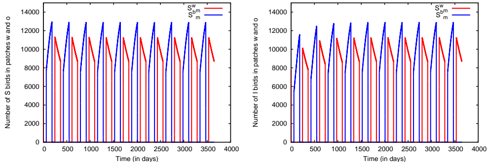
Figure 6: Number of susceptible migratory birds over 10 years in the absence of poultry. The left plot shows the situation when no infected migratory birds are introduced ( I_m^w(0) = 0 , S_m^w(0) = 8800 ) and the right one shows the situation when I_m^w(0) = 1000 , S_m^w(0) = 7800 . In both cases parameters are such as to result in evolution to a disease free periodic equilibrium. Here, \beta_m = 2.3 \times 10^{-5} \text{ day}^{-1} , r = 15,000 , \gamma = 0.0146 \text{ day}^{-1} , \mu_{ms} = 0.0022 \text{ day}^{-1} , and \mu_{mi} = 0.23 \text{ day}^{-1} . The death rates in flight are taken to be equal to those on land.
