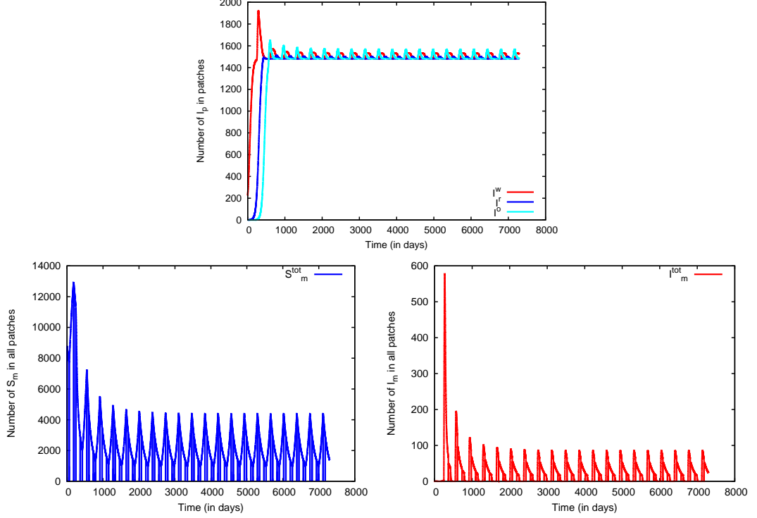
Figure 8: (top) Number of infected poultry on endemic farmed patches and (bottom) number of susceptible and infected migratory birds showing the persistence of the disease and convergence to periodic solutions. Here, I_m^w(0) = 0 , S_m^w(0) = 8800 , I_p^w(0) = 224 , N_p = 22,400 on all patches except the breeding patch assumed to be poultry free, \beta_m = 2.14 \times 10^{-5} \text{day}^{-1} , r = 15,000 , \gamma = 0.0146 \text{day}^{-1} , \mu_{ms} = 0.0022 \text{day}^{-1} , and \mu_{mi} = 0.23 \text{day}^{-1} , \mu_p = 0.4 \text{day}^{-1} , and \beta_p = 1.9 \times 10^{-5} \text{day}^{-1} .
