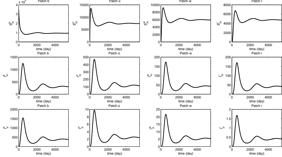
Figure 5: This figure shows that if inequalities (4.25), (4.27) and (4.28) do not hold, then the disease free equilibrium of system (2.4)-(2.5) loses its stability and the disease persists. Here, the parameter values are the same as in Fig. 4 except that \beta_m^b = 25 \times 10^{-7} , \beta_{mp}^b = \beta_{pm}^b = 5 \times 10^{-8} .
