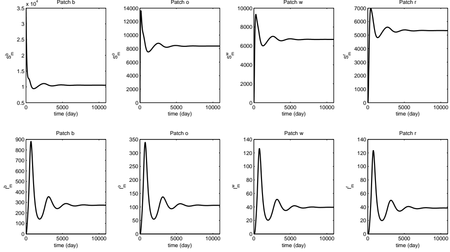
Figure 3: Stability with poultry absent. This figure demonstrates that if inequality (4.27) is not satisfied, there will be a disease outbreak. Here \beta_m^b = 25 \times 10^{-7} and \beta_m^j = 5 \times 10^{-7} for j = o, w, r .
