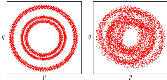
FIG. 2: (Color online) Plot of p versus q for the logistic map. (a) a = a_\infty ; (b) a = a_\infty + 0.001 . We used 5000 data points.
