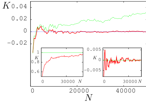
FIG. 1: (Color online) Plot of K as a function of N for the logistic map at a = a_\infty (continuous line, online red) and a = a_\infty + 0.001 (dashed line, online green). Although the value of K is small in both cases, the behaviour of K as a function of N distinguishes the two cases. The corresponding graphs for fully developed chaos at a = 3.99 and regular dynamics at a = 3.561 are shown in the left and right insets respectively.
