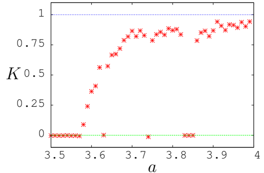
FIG. 3: (Color online) Plot of K versus a for the logistic map with 3.5 \leq a \leq 4 increased in increments of 0.01. We used 5000 data points. The horizontal lines indicate K = 0 and K = 1 .
