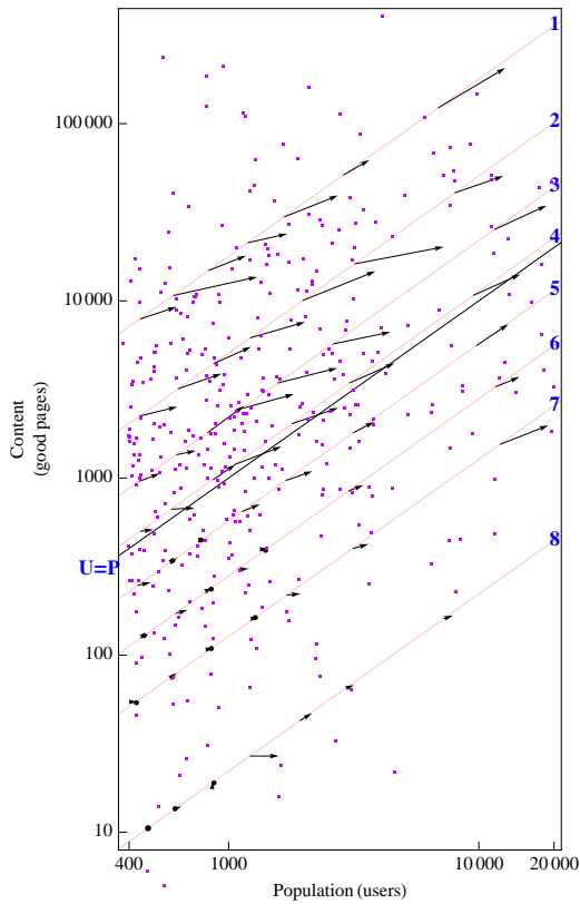
Figure 3: Phase diagram in the content/population space of wikis belonging to the clean dataset.
