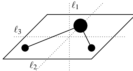
Figure 2: Axes for the XY_2 molecule
