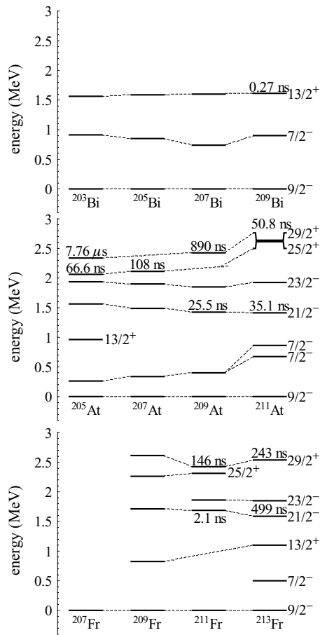
FIG. 8. Levels [12,14,16,18,21] in the odd Bi, At, and Fr isotopes indicative of the relative energies of the orbitals. The 29/2^+ and 25/2^+ states are likely members of the \pi i_{13/2} \otimes \pi(h_{9/2})^2 configuration. The 23/2^- and 21/2^- maximally aligned states presumably have the \pi f_{7/2} \otimes \pi(h_{9/2})^2 and \pi(h_{9/2})^3 configurations, respectively.
