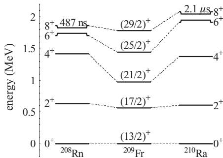
FIG. 10. Comparison of similar configurations in the N = 122 Rn [15], Fr, and Ra [36] isotopes.
