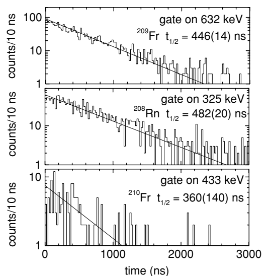
FIG. 4. Time relative to implantation for several gamma rays measured at the focal plane. The solid line shows a weighted least squares fit to decay spectrum of isomeric gamma rays: 632 keV ( ^{209}\text{Fr} ), 325 keV ( ^{208}\text{Rn} ), and 433 keV ( ^{210}\text{Fr} ).
