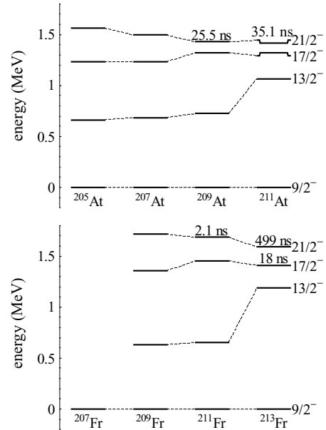
FIG. 9. Comparison of level spacings of the (h_{9/2})^3 configurations in the odd-At [14,16,18] and odd-Fr [21] isotopes.
