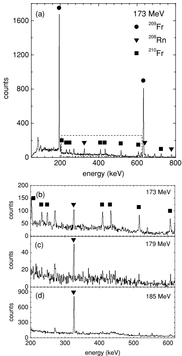
FIG. 3. Gamma ray spectra obtained at the focal plane at 173, 179, and 185 MeV. Top: Portion of spectrum (a) of delayed gamma rays measured at the focal plane at a beam energy of 173 MeV. The spectrum is dominated by the 194 and 632 keV gamma rays belonging to ^{209}\text{Fr} . Bottom: Portion of the spectrum indicated by dashed box in (a) between the 194 and 632 keV gamma rays at (b) 173, (c) 179, and (d) 185 MeV beam energies. The varying strengths of the 3, 4, and 5 particle channels are evident from the relative intensities of the corresponding gamma rays.
