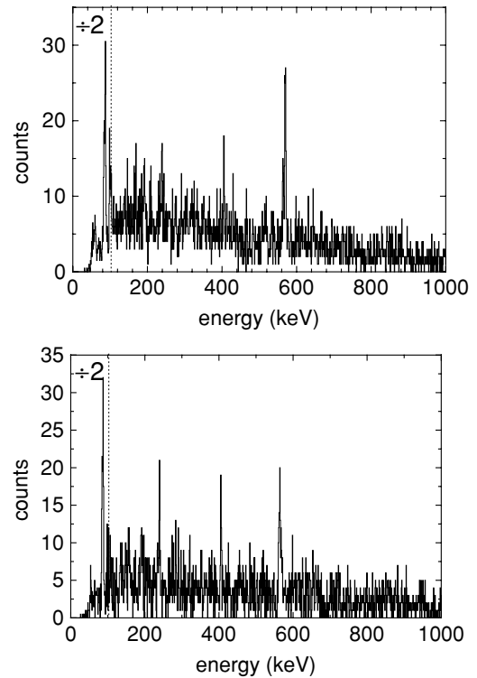
FIG. 5. Gate on 632 keV isomeric transition (top) shows prompt gamma rays in coincidence. Gates in the recoil-gamma-gamma matrix, such as the gate on the 568 keV transition (bottom), have been used for building the level scheme.
