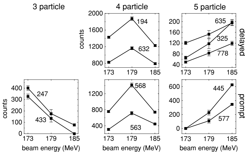
FIG. 2. Excitation function measured in this work for the 3, 4, and 5 particle channels. Top panels show gamma rays detected at the focal plane. Bottom panels show gamma rays detected at the target position. The 194, 632, 568, and 563 keV transitions belong to ^{209}\text{Fr} . The 635, 325, 778, and 577 keV transitions belong to ^{208}\text{Rn} . For details, see text. (Note the suppressed zero in some of the plots.)
