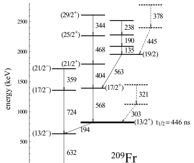
FIG. 6. Level scheme for ^{209}\text{Fr} obtained in this work. Dashed lines indicate tentative assignments.
