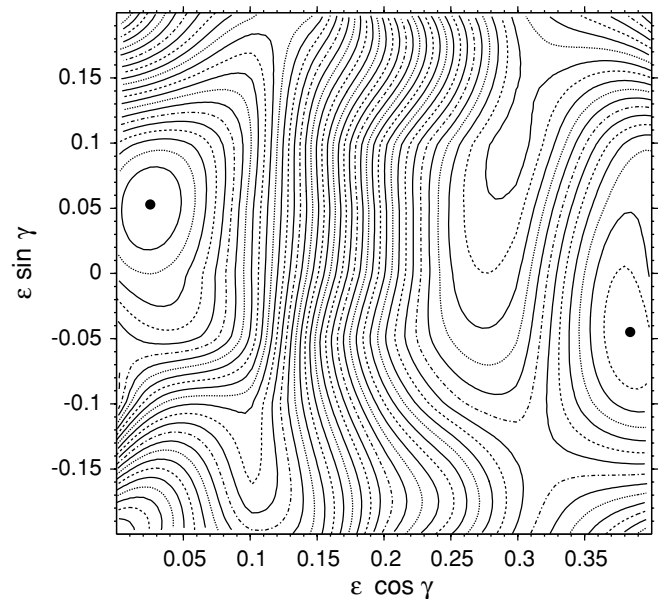
FIG. 7. Calculations done using the ultimate cranked model [29] with \hbar\omega = 0.23 MeV for positive parity proton and neutron excitations, shown with contours of 200 keV. They show two minima at low excitation energies: One very deep, slightly oblate minimum (left) and one higher-lying, strongly prolate minimum (right).
