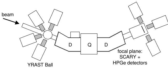
FIG. 1. The beam is incident (from the left of this figure) on a target centered at YRAST Ball. The recoils are then focused to the focal plane by setting the fields of two dipole magnets and one quadrupole magnet. Recoiling nuclei are detected in SCARY, an array of 30 solar cells. Prompt gamma rays are detected using YRAST Ball, and delayed gamma rays are detected using Ge detectors around the focal plane.
